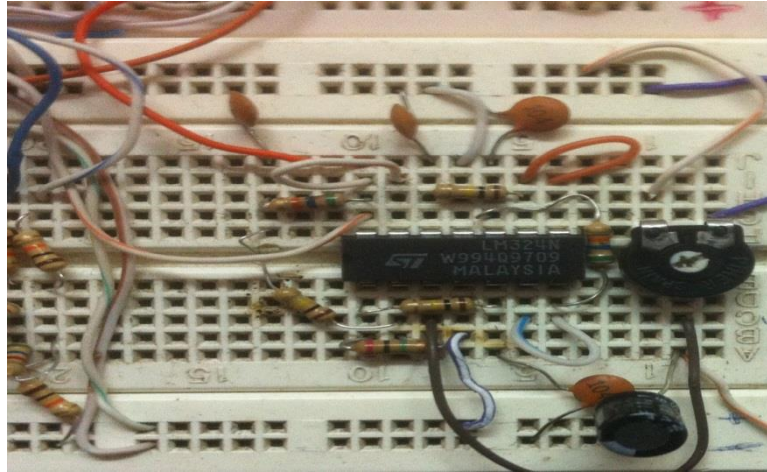
Figure c5 :Bubba oscillator
